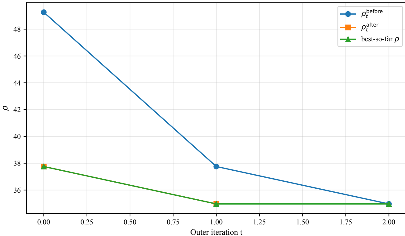
Alg2 outer residual history
